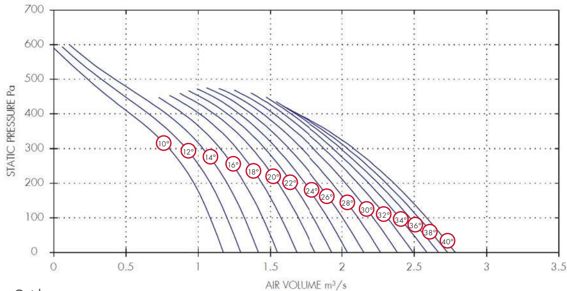
BIFA40 - 1 & 3 Phase - 2 Pole
