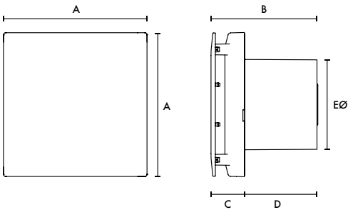
Closed Grille
