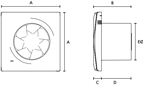
Open Grille
