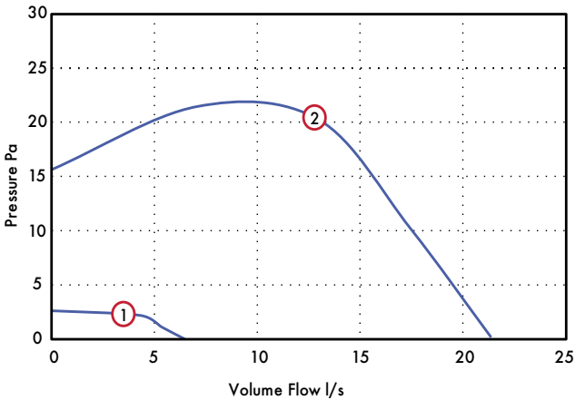
Open Grille
